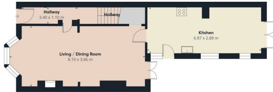
Ground Floor
